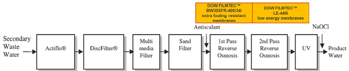
Figure 2. AITASA Water Reclamation Plant process scheme.
