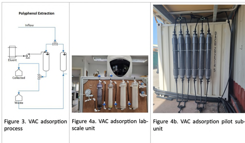
Figure 46. VAC adsorption process, VAC adsorption laboratory scale unit and VAC adsorption pilot sub-unit.
