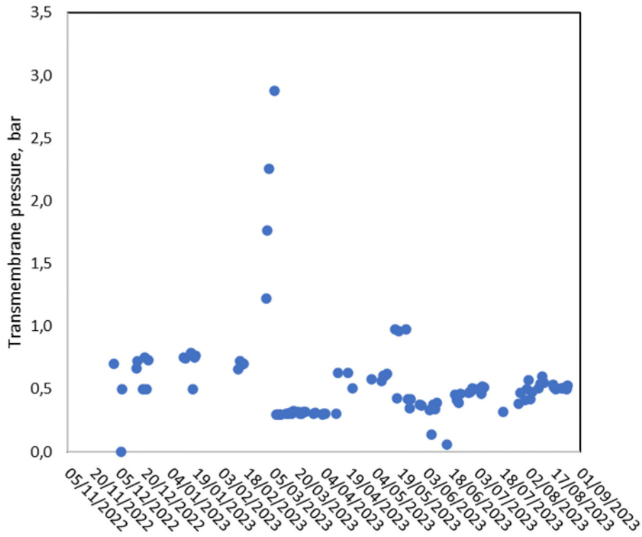
Figure 9. Ultrafiltration transmembrane pressure.
