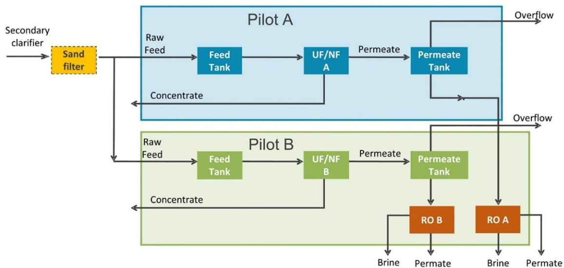
Figure 124. Pilot container A and B with pre-treatment, tanks, membrane units and water streams.
