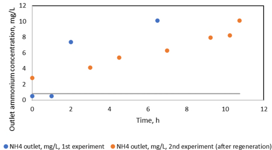
Figure 16. Ammonium adsorption on zeolites.
