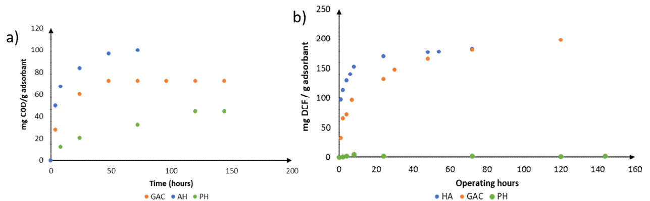
Figure 35. Kinetic adsorption tests for a) COD removal from wastewater, and b) DCF by using GAC, AH and PH. COD concentration was 84 mg/l for GAC test, 70 mg/l for AH test and 65 mg/l for PH test. Diclofenac concentration was 60 mg/l for all tests. Adsorbents dosages: 0.1 g of GAC, 0.1 g of AH and 0.05 g of PH.
