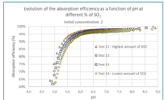
Figure 121. Evolution of the absorption efficiency as a function of pH for different percentage of SO 2 at the second concentration tested in the absorption liquid
