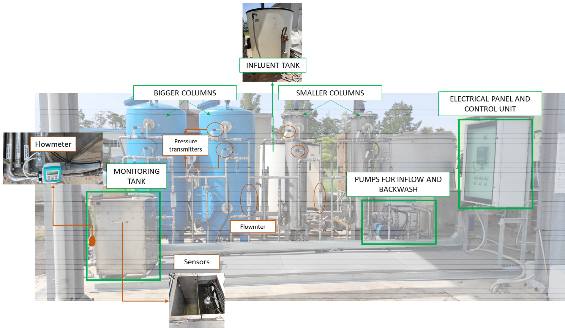
Figure 30. Adsorption pilot plant.
