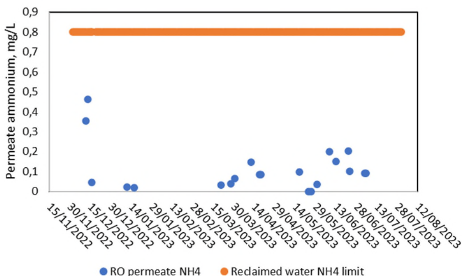
Figure 14. Reverse Osmosis ammonium concentration in permeate.
