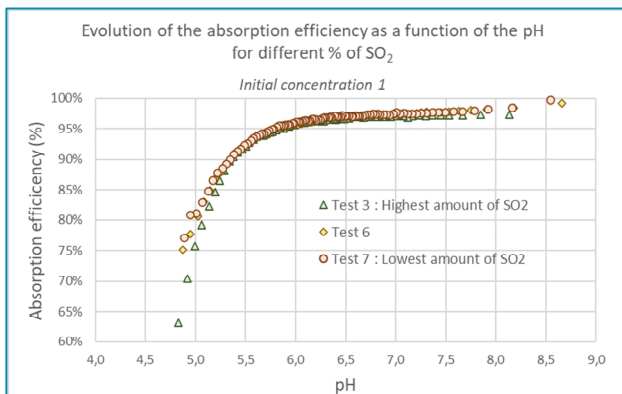
Figure 120. Evolution of the absorption efficiency as a function of pH for different percentage of SO 2 at the first concentration tested in the absorption liquid
