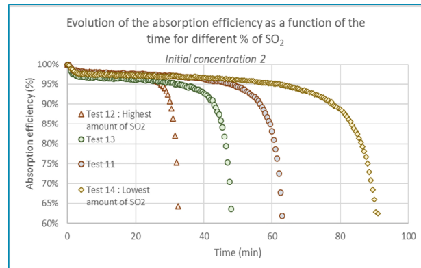
Figure 118. Evolution of the absorption efficiency as a function of the time for different percentage of SO 2 at the second concentration tested in the absorption liquid
