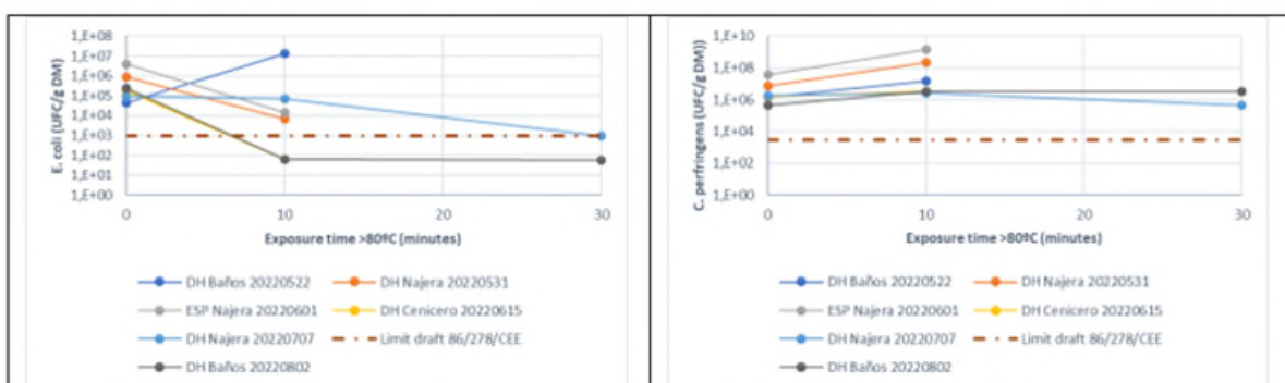
Figure 91. Evolution of Escherichia coli and Clostridium perfringens in sludge samples exposed to a thermosolar-based drying system at temperatures >80°C.
