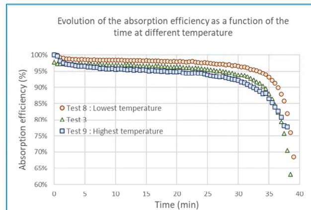
Figure 122. Evolution of the absorption efficiency as a function of the time at different temperature.
