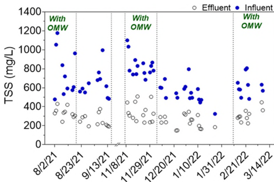
Figure 98. Total suspended solids (TSS) as a function of time after the AAT in the Karmiel system.
