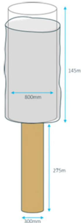
Figure 25. Schematic representation of the deepening drilling as carried out at the TRIAS Westland site.
