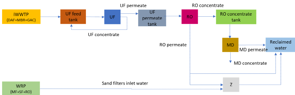
Figure 5. CS1 pilot plant process scheme.
