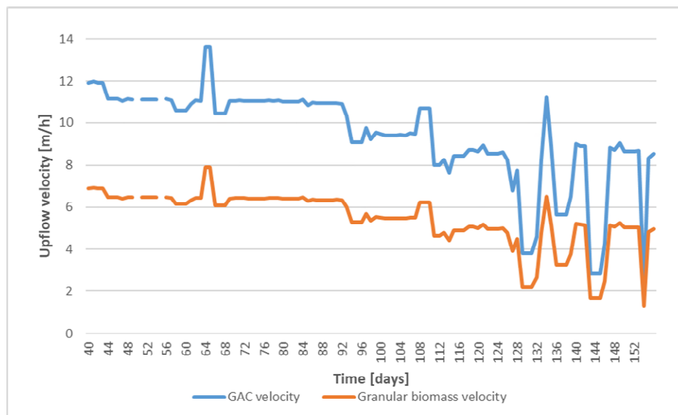
Figure 85. Evolution of upflow velocity in the ELSAR pilot plant.
