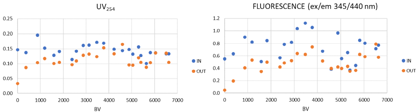
Figure 41. UV and Fluorescence laboratory measurements on influent and effluent samples from the pilot plant.
