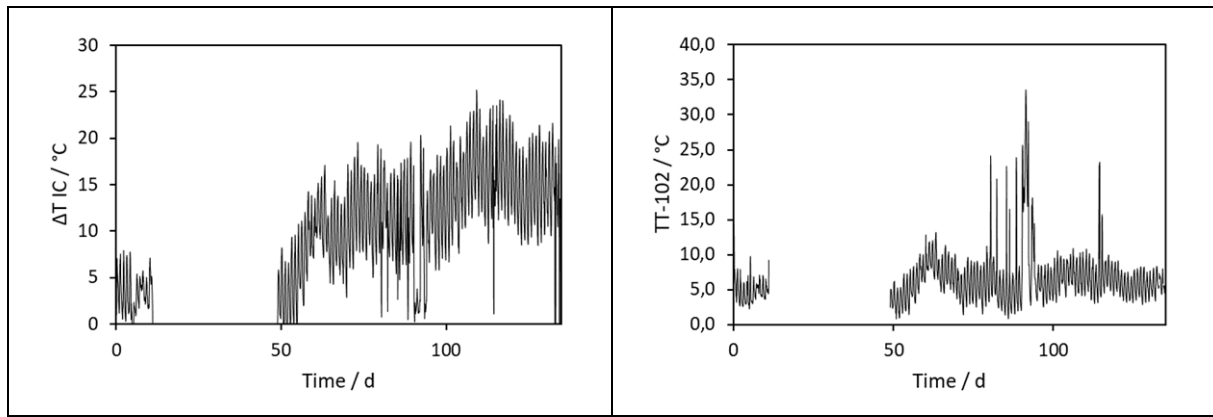
Figure 88. Evolution of temperature difference of the biogas before and after the heat exchanger (left) and temperature of the biogas after the heat exchanger (right) in the solid oxide fuel cell pilot plant (hourly registration).
