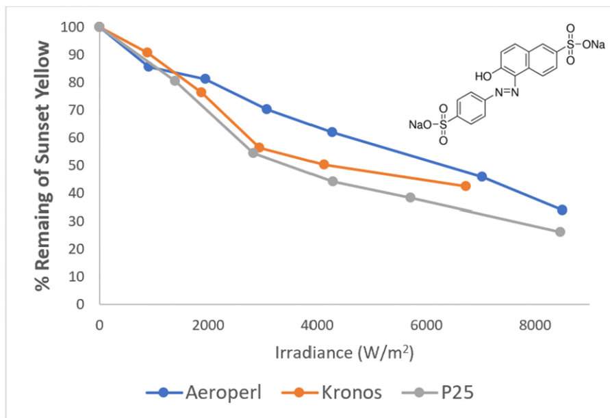
Figure 53. Degradation of a model organic compound using the CPC solar reactor.
