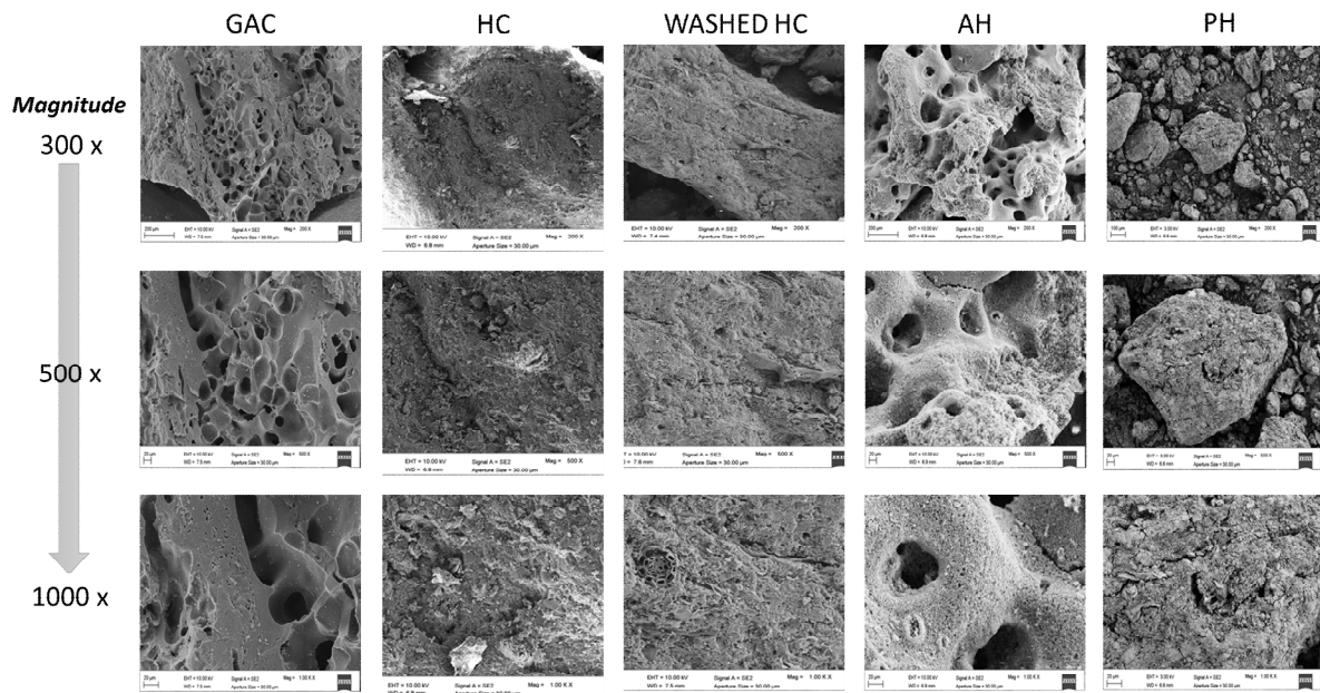
Figure 34. SEM analysis of commercial Granular Activated Carbon (GAC), Hydrochar (HC), washed Hydrochar, Activated Hydrochar (AH) and Pyrolyzed Hydrochar (PH).
