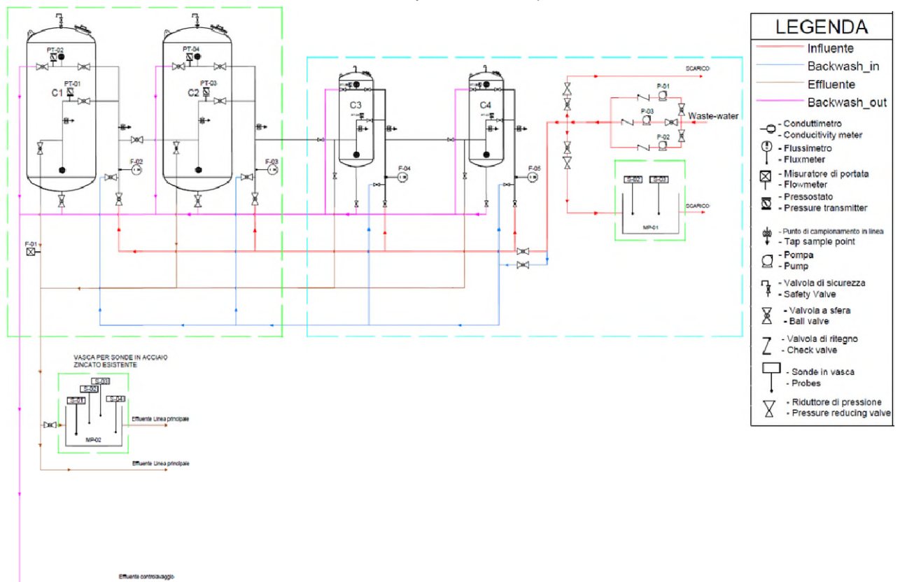
Figure 29. PID of the adsorption pilot plant.
