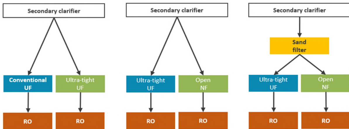
Figure 126. Tested treatment trains.
