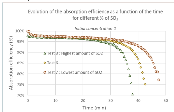
Figure 119. Evolution of the absorption efficiency as a function of the time for different percentage of SO 2 at the first concentration tested in the absorption liquid
