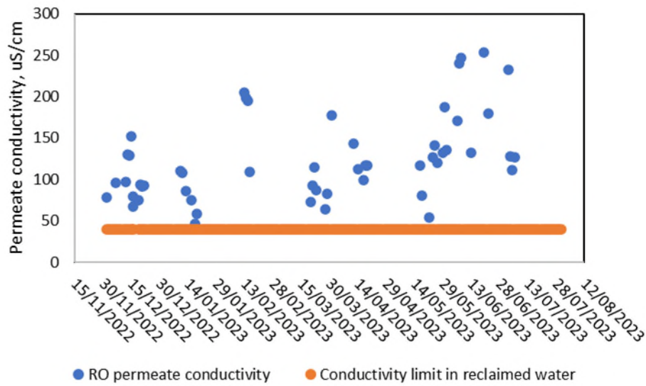
Figure 15. Reverse Osmosis conductivity concentration in permeate.
