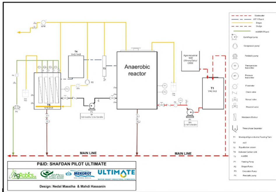
Figure 95. PID of the Shafdan pilot plant system.
