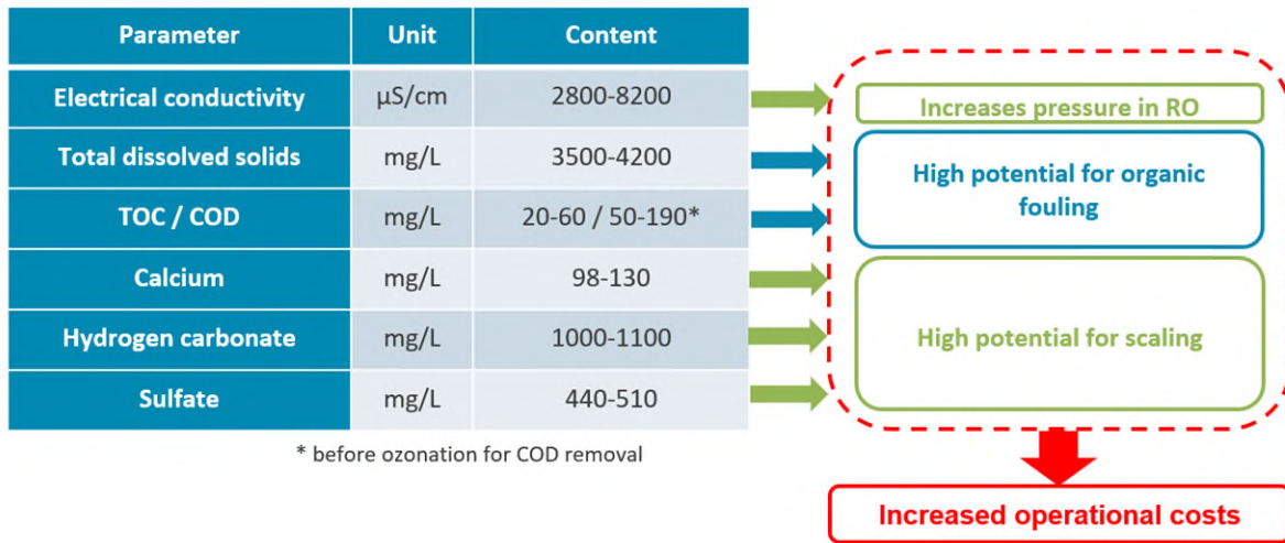
Figure 123. Composition of the outlet of the secondary clarifier of the municipal WWTP and upstream of the final ozonation unit.
