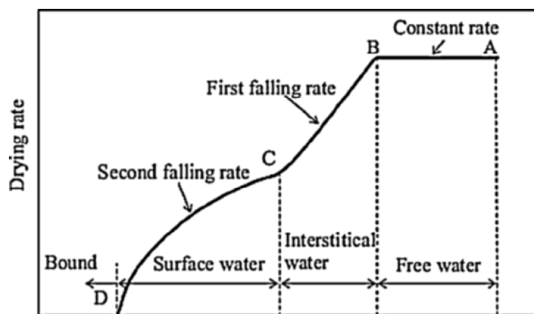
Figure 90. Correlation between drying rate and type of water bindings in biosolids [5].
