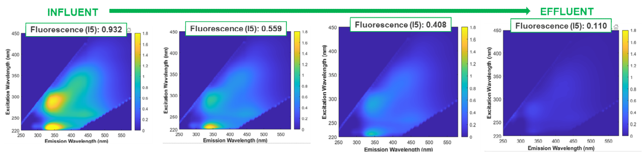
Figure 32. Fluorescence spectra of influent, effluent, and mixed (influent/effluent) samples collected in the monitoring tank of the adsorption pilot plant.
