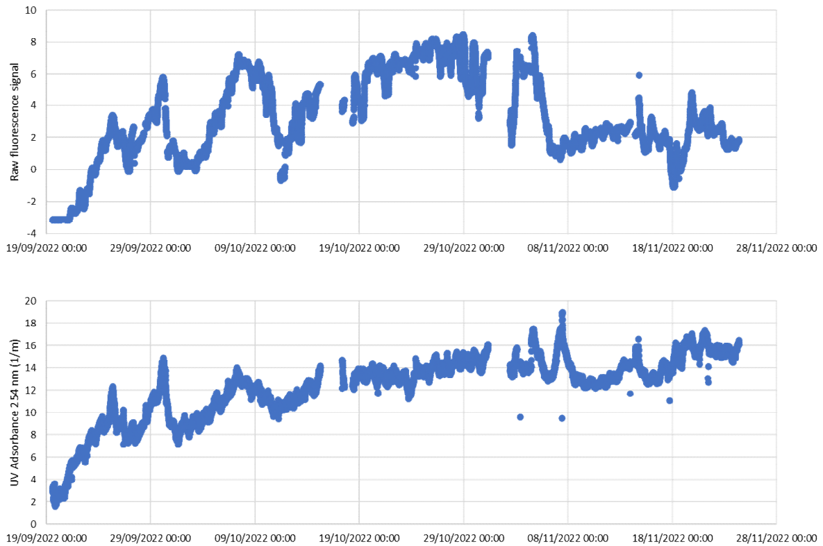
Figure 40. UV and Fluorescence trend.
