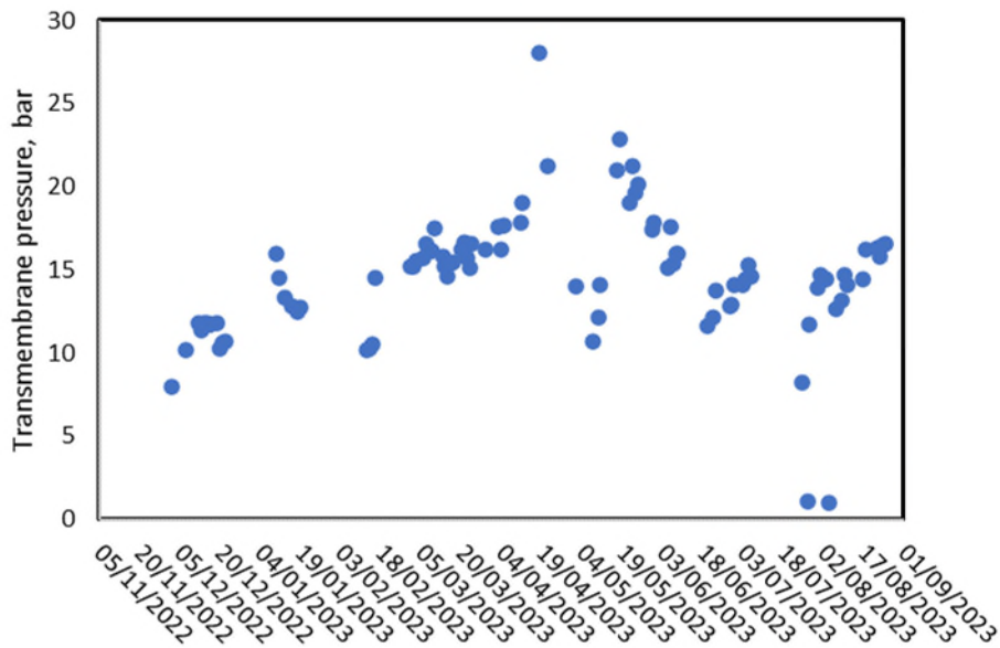
Figure 12. Reverse Osmosis transmembrane pressure.
