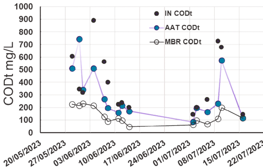
Figure 99. Total COD in the inlet, outlet of AAT system and the final outlet of the AnMBR system
