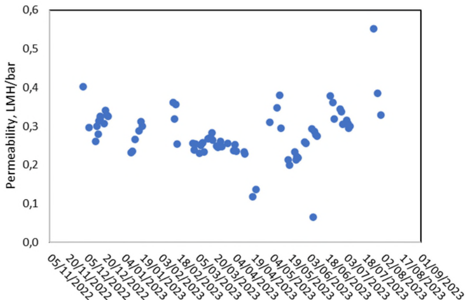
Figure 13. Reverse Osmosis permeability.
