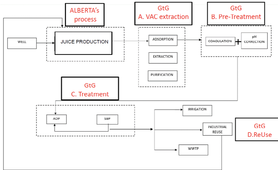
Figure 45. Layout of the pilot process deployed at Alberta S.A.
