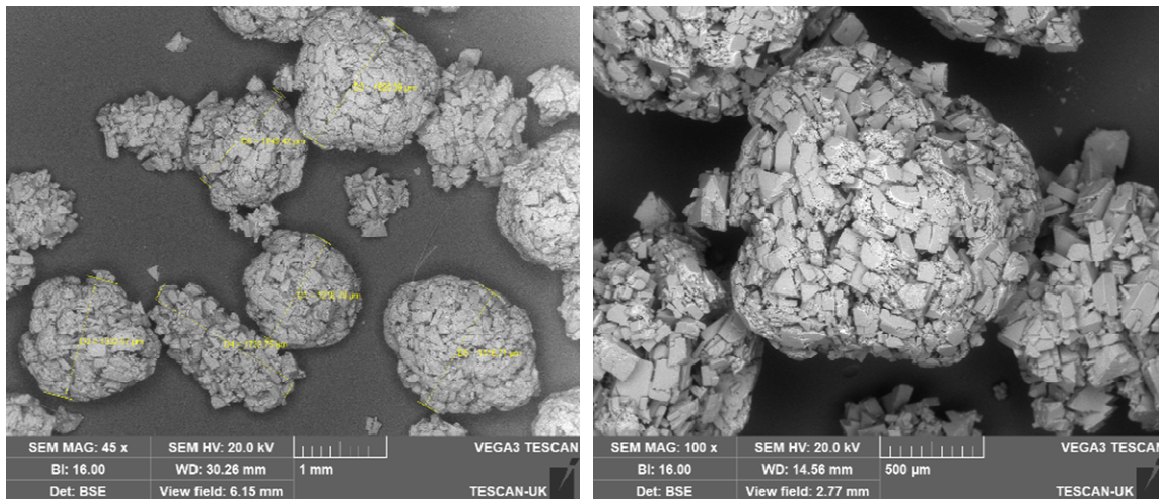
Figure 109. Scanning electron microscope images of the struvite pellets harvested after the first trial (pH = 8.3, Mg:P 1.3:1).
