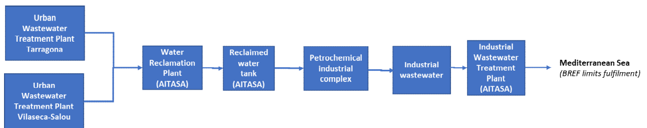
Figure 3. Scheme of the pre-existing system and the partners of the symbiosis before the start of ULTIMATE.
