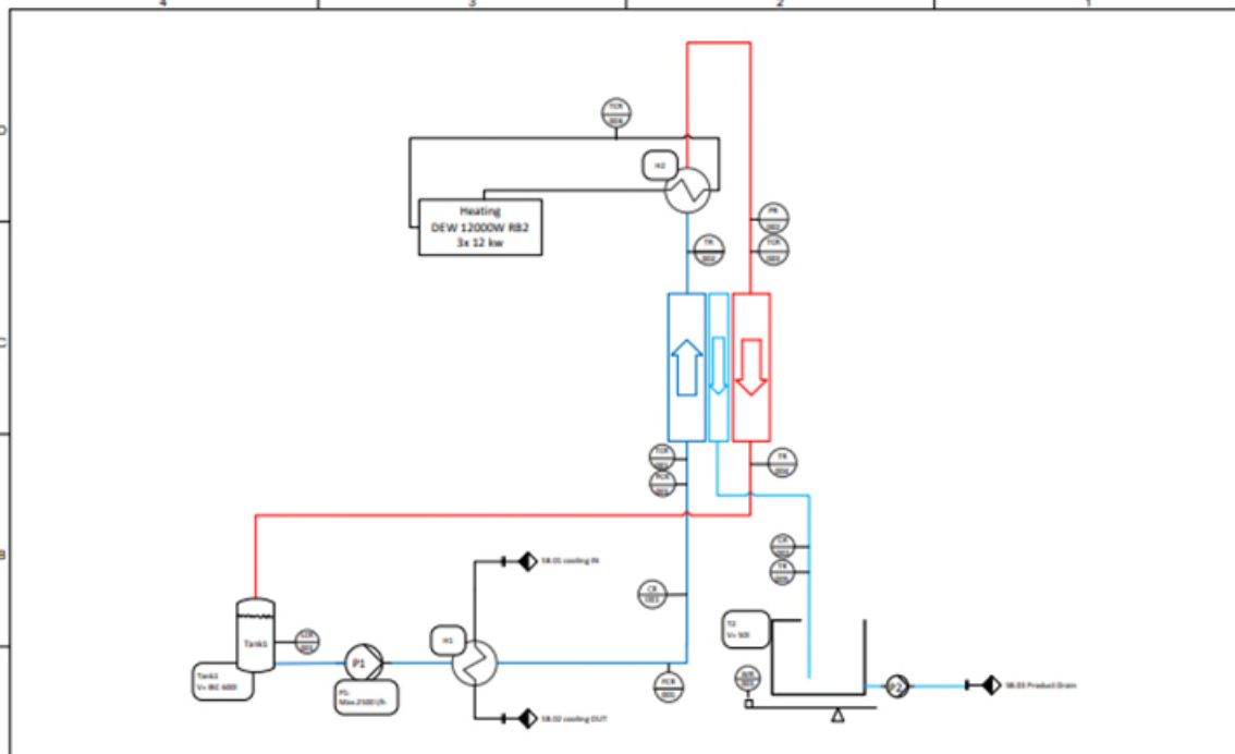
Figure 8. Membrane distillation pilot plant PID scheme.
