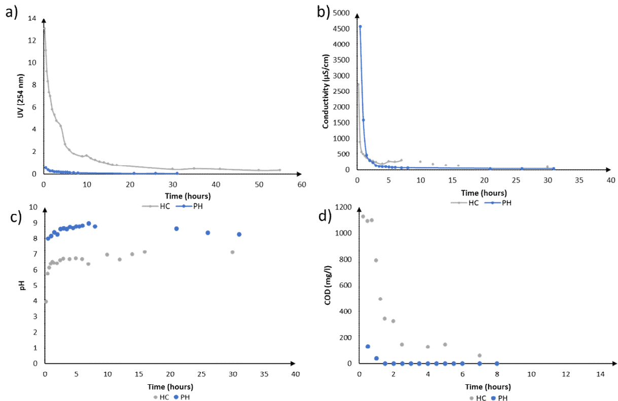
Figure 33. Washing tests in columns filled with Hydrochar (HC) and Pyrolyzed Hydrochar (PH). Monitored parameters included UV absorbance at 254 nm (a), conductivity (b), pH (c) and COD (d).
