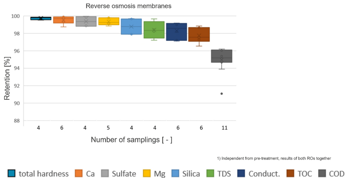
Figure 128. Retention of different water quality parameters using reverse osmosis.
