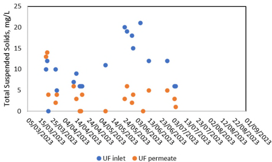
Figure 11. Suspended solids removal at the UF inlet and permeate.
