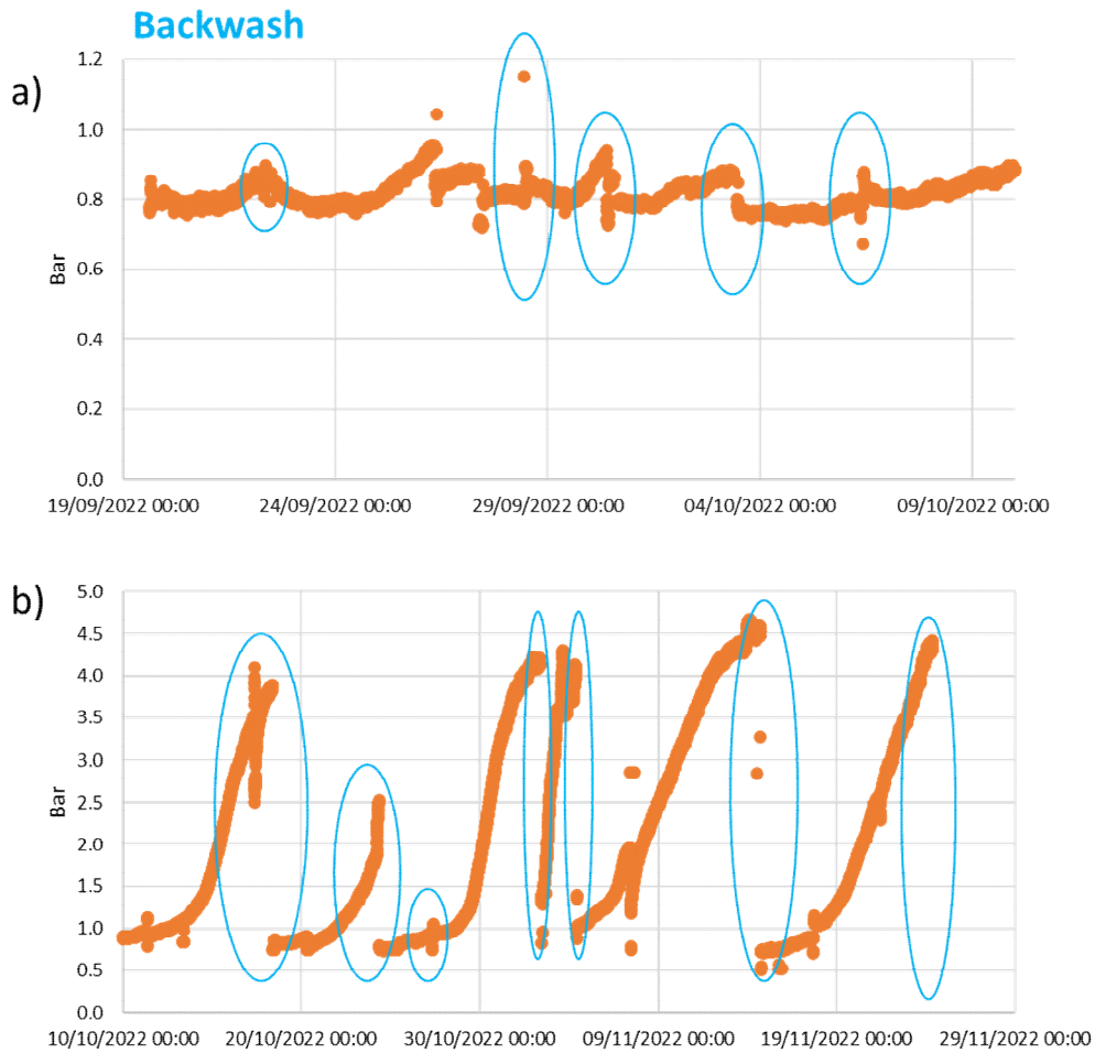
Figure 38. Pressure trend before (a) and after (b) maintenance of the relief valve.
