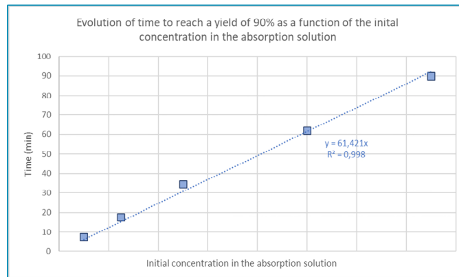
Figure 116. Evolution of time to reach an absorption efficiency of 90 % as a function of the initial concentration.
