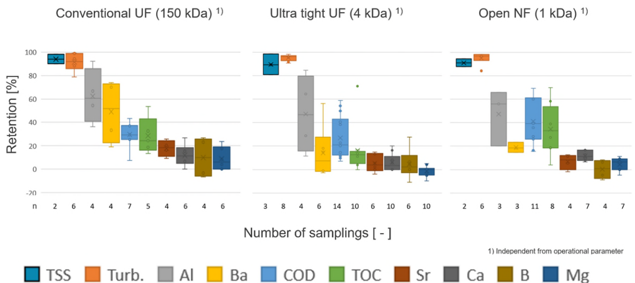
Figure 127. Retention of selected water quality parameters using different membrane types.
