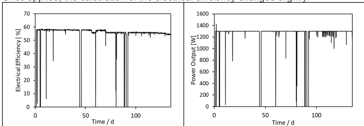
Figure 86. Evolution of electrical efficiency and power output in the solid oxide fuel cell (hourly registration).
