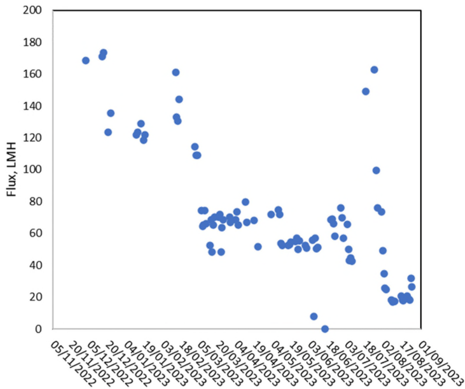
Figure 10. Ultrafiltration flux.
