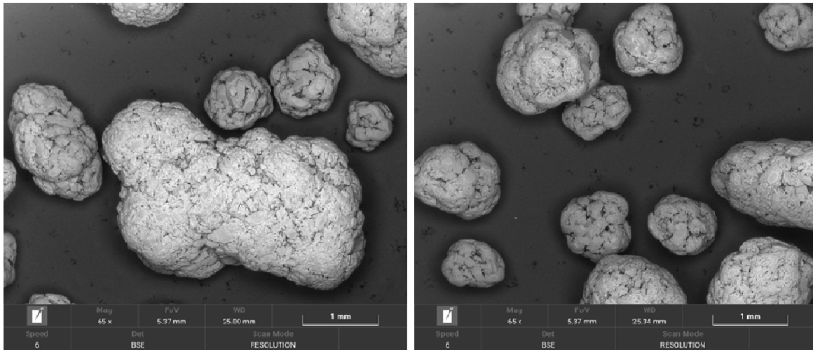
Figure 110. Scanning electron microscope images of the struvite pellets harvested in the later trial (pH = 7.7-8.5, Mg:P 1:1).
