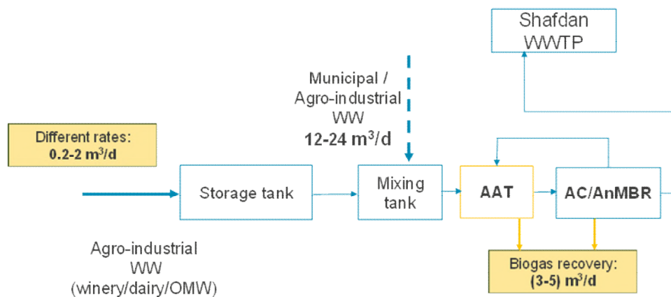
Figure 94. Schematic description of Shafdan system.
