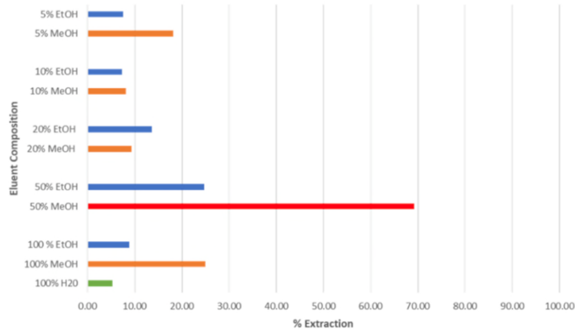
Figure 51. Effect of various extraction solvents in the recovery of VACs from sorbent material.
