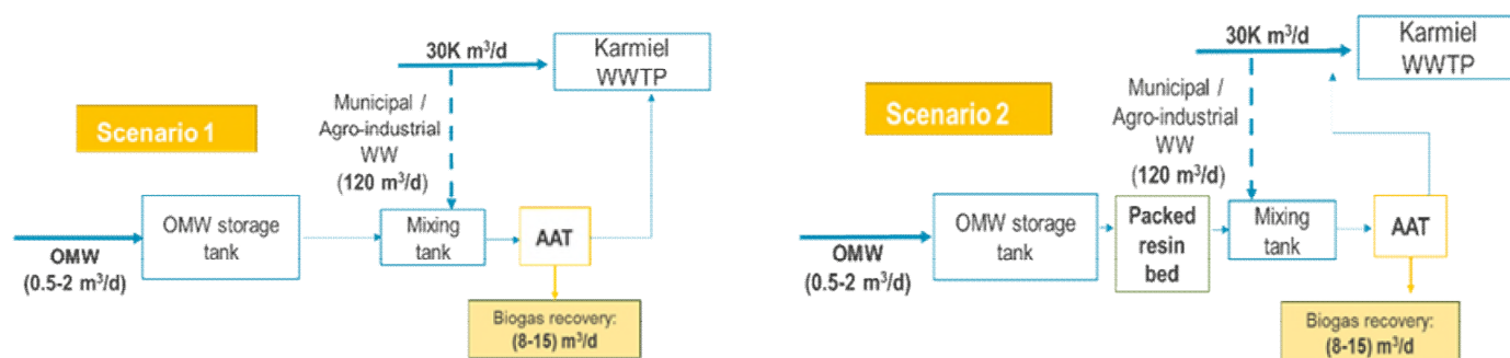
Figure 93. Schematic description of biogas production (Scenario 1) and polyphenols recovery (Scenario 2).
