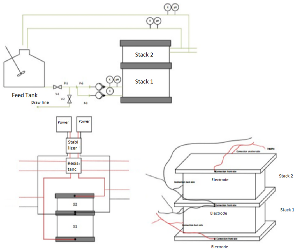
Figure 20. PID of the ED stack and pilot installation.
