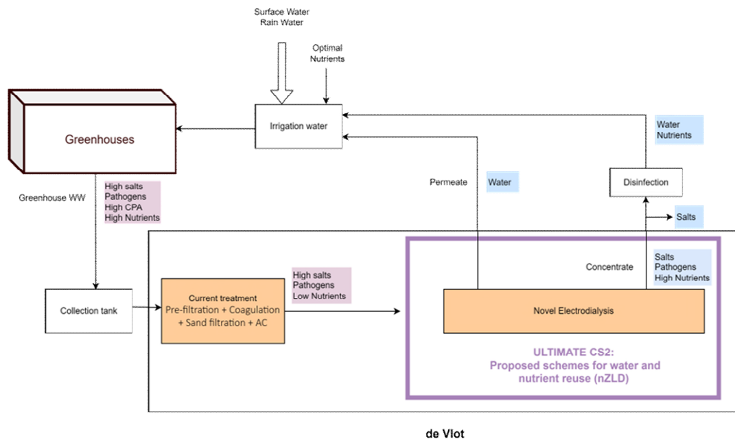
Figure 19. The proposed technological solutions from ULTIMATE in the water system at De Vlot (ULTIMATE addition indicated in purple).
