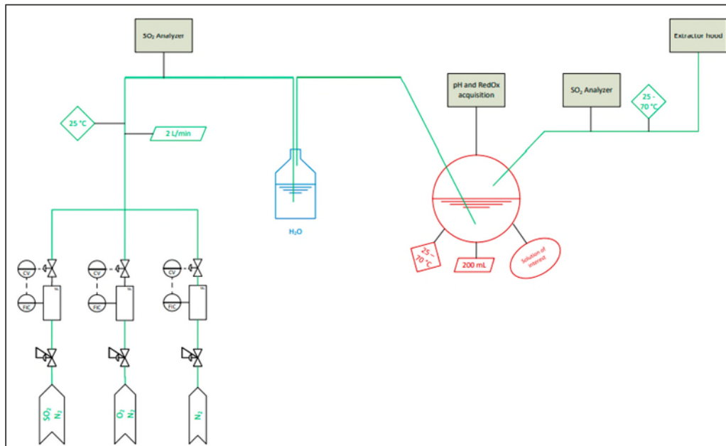
Figure 114. Diagram of the laboratory pilot.
