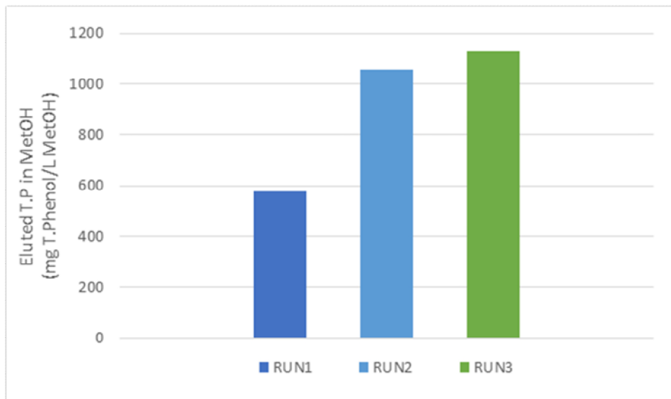
Figure 101. Total polyphenols from resin extraction in methanol (Concentration adsorption on the resin).
