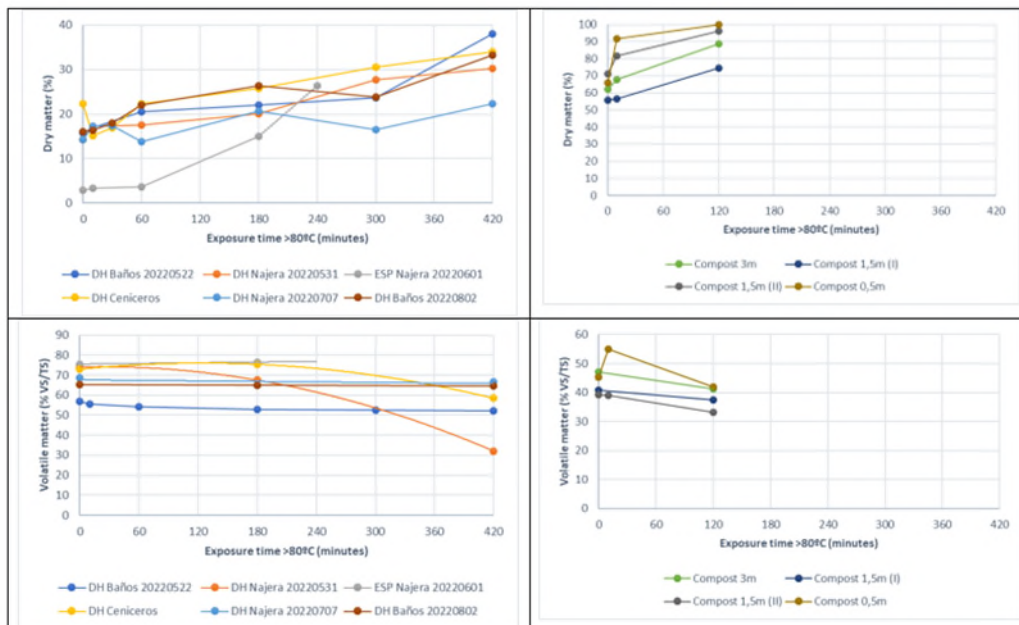
Figure 89. Top: Dry matter evolution in thermosolar batch tests with sludge (left) and compost (right). Bottom. Volatile matter evolution in thermosolar batch tests with sludge (left) and compost (right). DH = dewatered WWTP sludge; ESP = thickened sludge; Compost samples: “m” means month of composting age.
