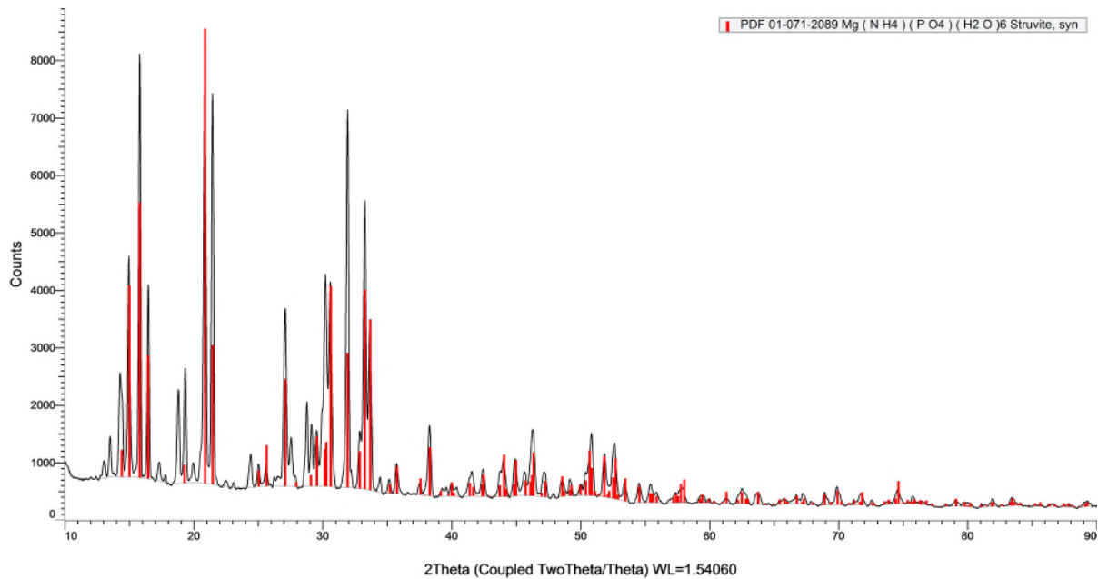
Figure 111. Example of X-ray diffraction spectrum for the pellets recovered from the reactor (black) matching closely the standard for struvite (red).
