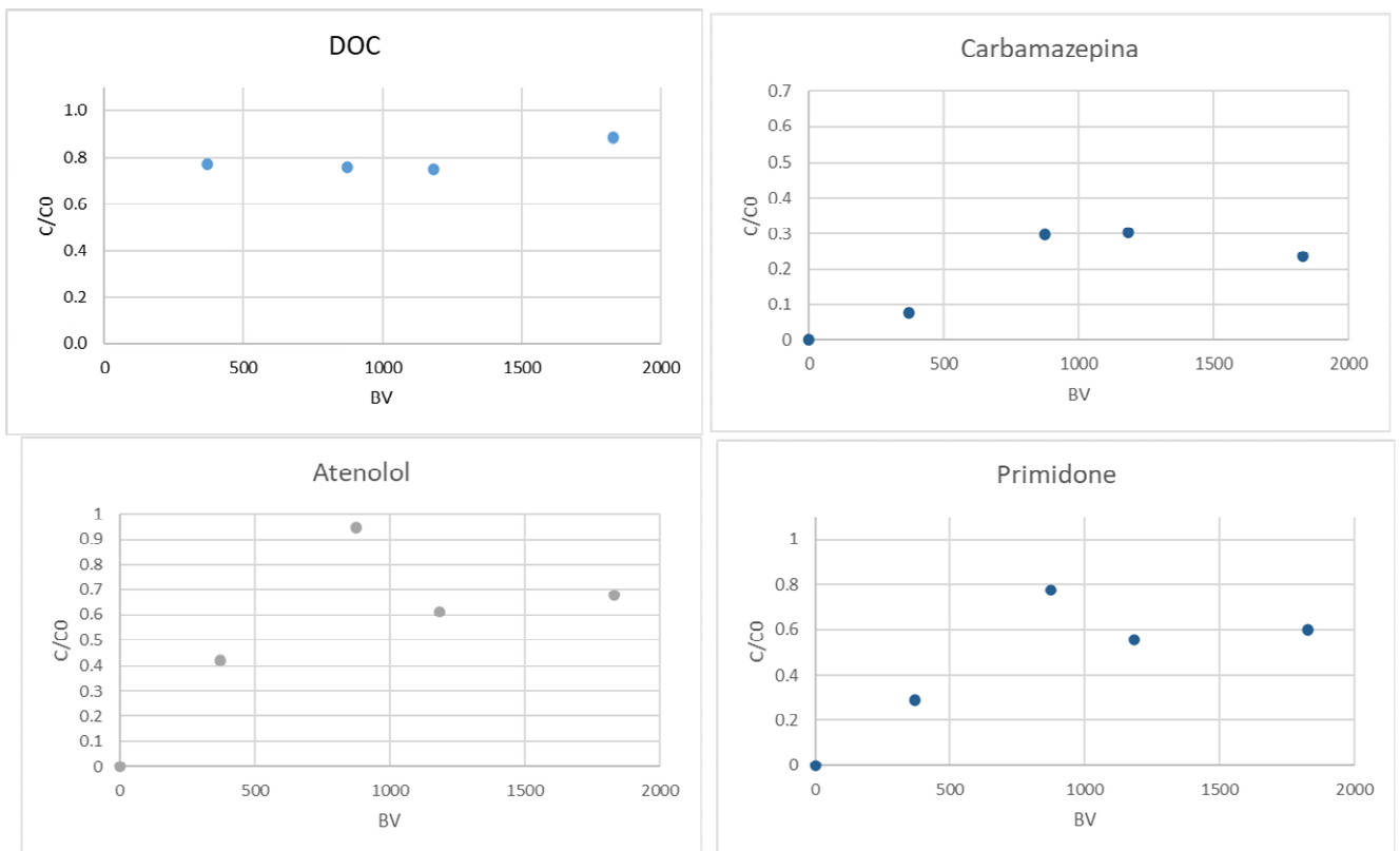
Figure 43. Monitored breakthrough for DOC and some emerging contaminants at the adsorption pilot system.
