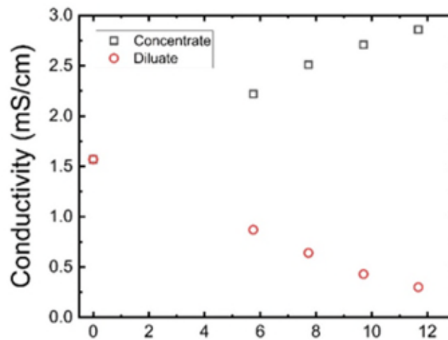
Figure 24. Change in conductivity over different voltages in the diluate and concentrate for the synthetic greenhouse wastewater CED pilot runs.
