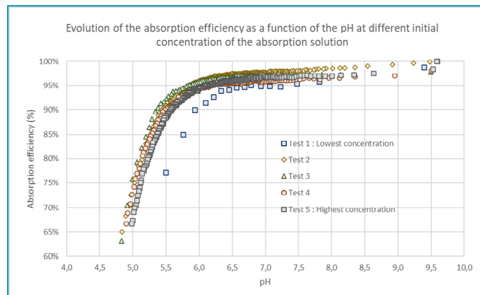
Figure 117. Evolution of the absorption efficiency as a function of the pH.
