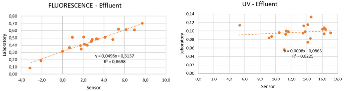
Figure 42. Comparison between laboratory and sensors measurements of fluorescence at ex/em 325/445 nm and UV absorbance at 254 nm.
