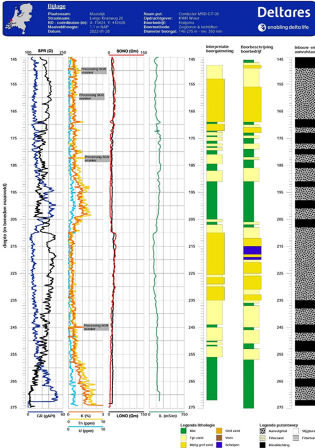
Figure 27. Lithological interpretation and well completion information from 145 to 275 m depth, based on the logging data and cuttings description.
