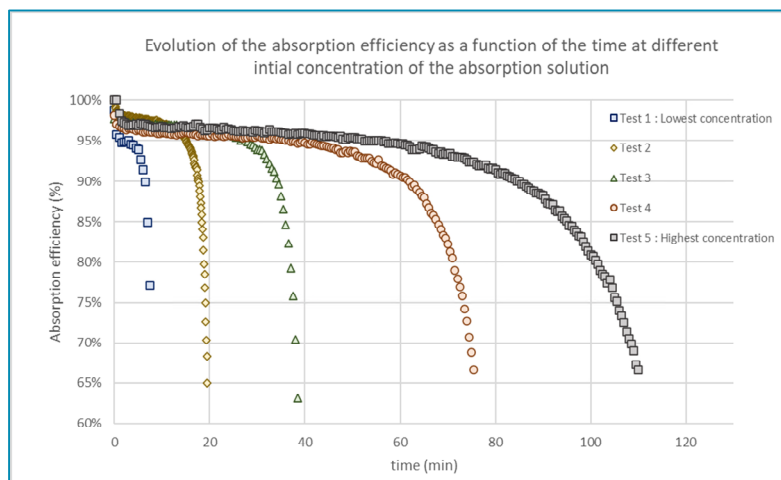
Figure 115. Evolution of the absorption efficiency as a function of the time
