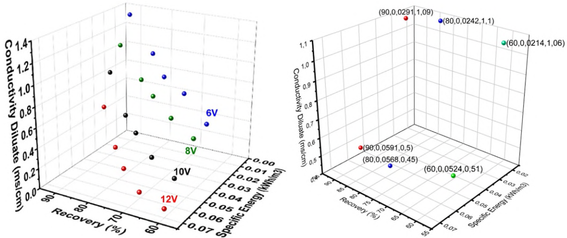
Figure 23. Specific energy consumption (kWh/m 3 ) as a function of recovery (%) and conductivity of the recovered water (mS/cm) for synthetic (left) and real (right) greenhouse wastewater experiments.
