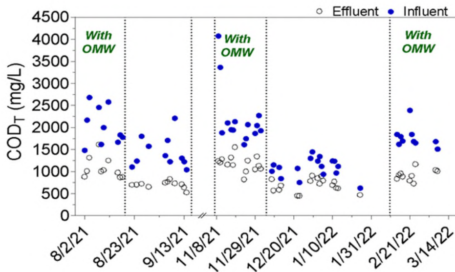
Figure 96. Total COD as a function of time after the AAT at the Karmiel system.
