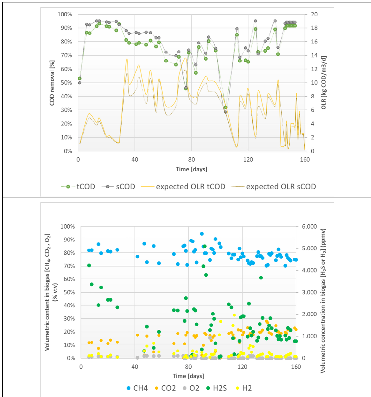
Figure 84. Evolution of COD removal and organic loading rate (top) and component concentration in biogas (bottom) in the ELSAR pilot plant.
