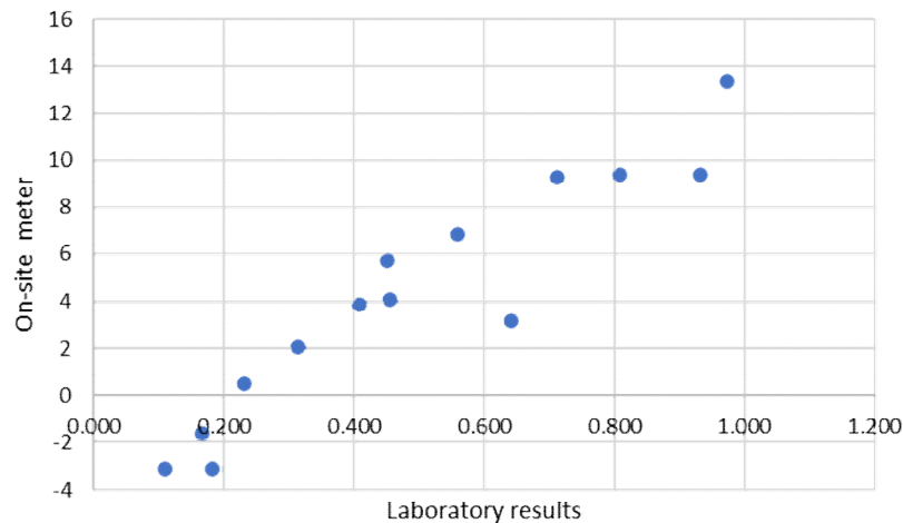
Figure 31. Calibration curve of fluorescence meter.
