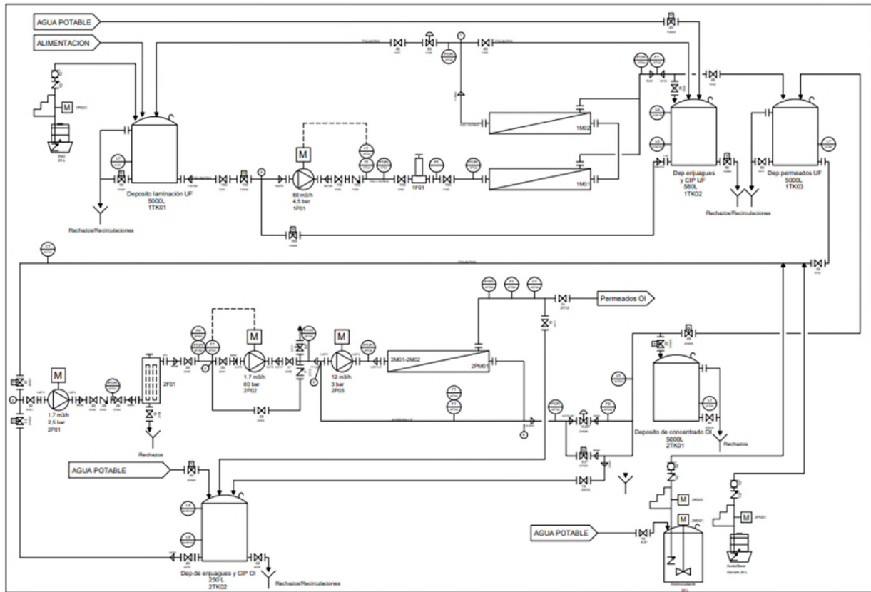
Figure 7. Ultrafiltration and batch reverse osmosis pilot plant PID scheme.
