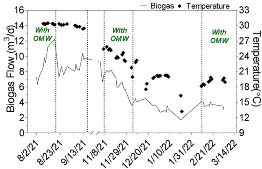
Figure 97. Biogas flow and temperature as a function of time from the AAT at the Karmiel system.
